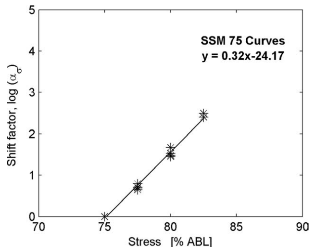
Figure 28 Eyring plot of SSM curves at starting reference load 75% ABL for Kevlar 49.
