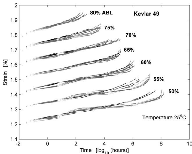
Figure 26 All SIM (gray) and SSM (black) master curves for Kevlar 49.
