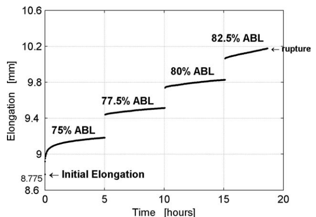
Figure 20 Elongation versus time curve.
