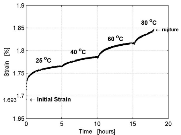
Figure 11 Strain versus time curve
